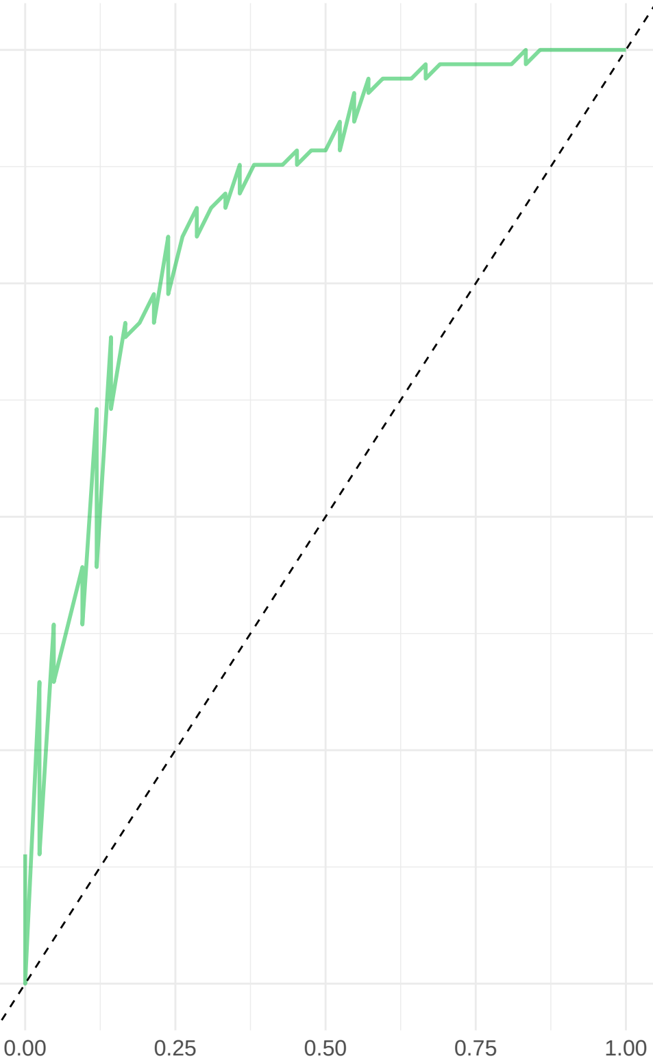
Bidirectional (AUC = 0.835)
